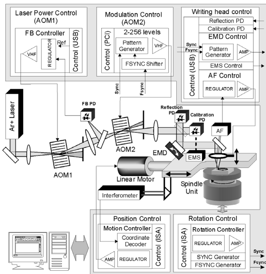
Fig. 4. Circular laser writing system
