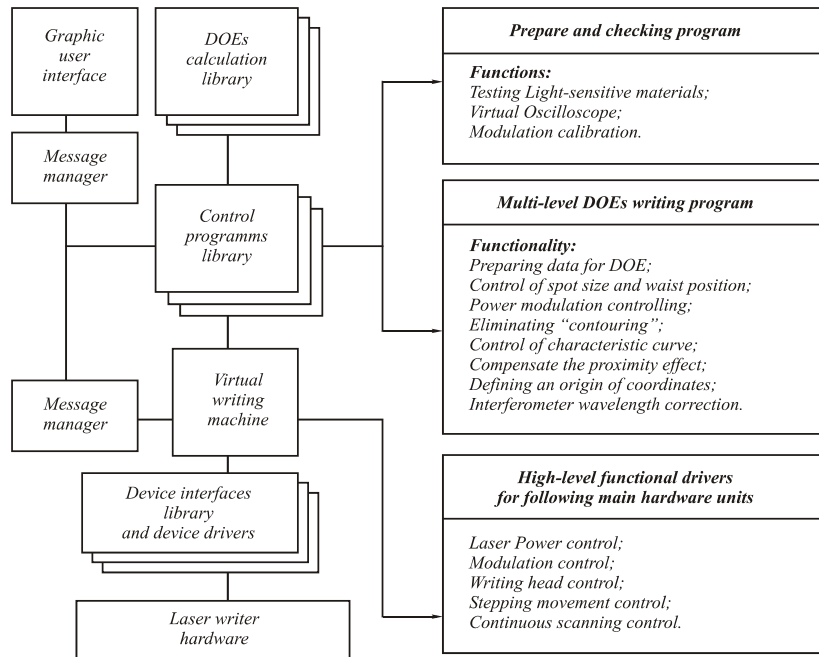
Fig. 15. Hierarchical modular structure of CLWS software environment
